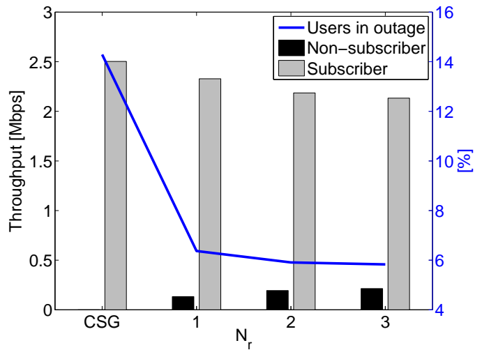
Fig. 4. Average throughput per user in a small residential scenario where 30% of the houses contains an OFDMA femtocell with 3 subscribers that request an intense data service. There are also 5 outdoor non-subscribers requesting a throughput between 80 and 450 kbps for video service. The system-level simulation is based on Monte-carlo snapshots.
