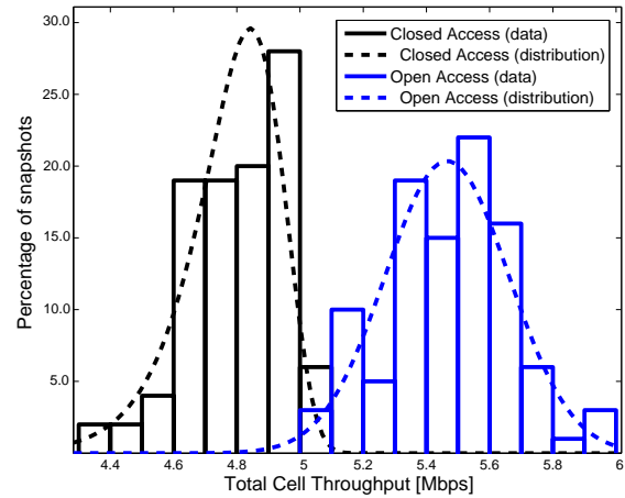
Fig. 3. Total downlink network throughput in a residential (200 x 100 m) area covered by 22 OFDMA femtocells and 1 macrocell (10 MHz bandwidth). Each house hosting a femtocell contains 2 indoor users demanding 128 kbps each. Furthermore, 10 macro users were located outdoors demanding 64 kbps each. The system-level simulation is based on Monte Carlo snapshots.
