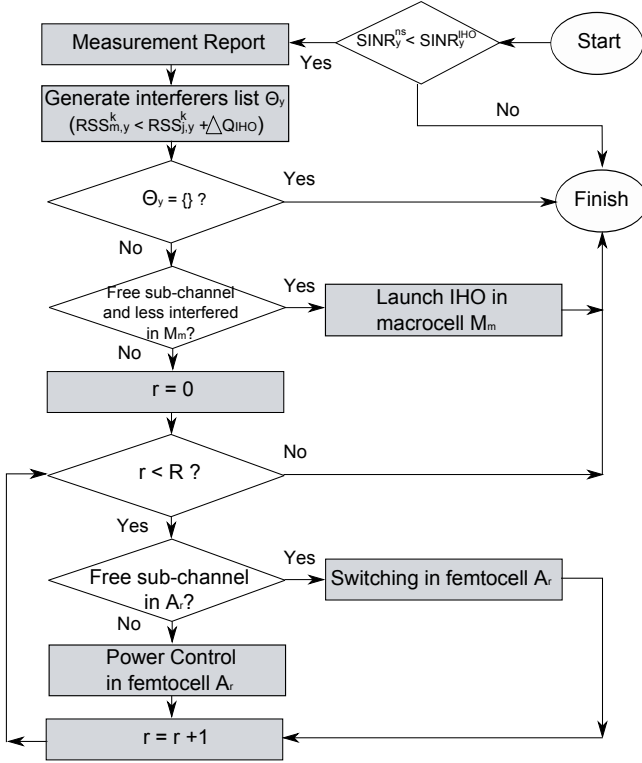
Figure 1: Intracell HandOver approach.
