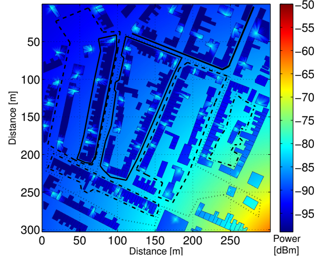
Figure 3: Received power per OFDMA sub-carrier (OFDMA-512 system) in a residential area covered by 1 macrocell and 64 femtocells. Each femtocell premises contains several indoor users, while 8 pedestrian users are located outdoors, being their routes also indicated.
