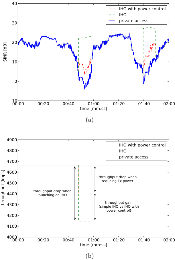
Figure 5: SINR level of a mobile non-subscriber.
