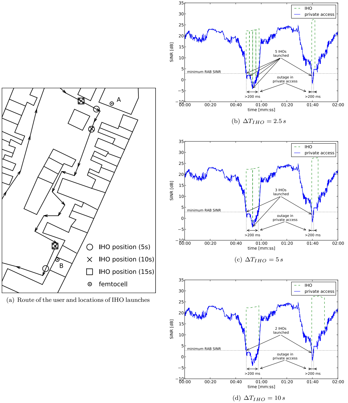
Figure 4: Performance comparison of CSG and IHO for a mobile non-subscriber ( \Delta Q_{IHO} = 3 \text{ dB} ).
